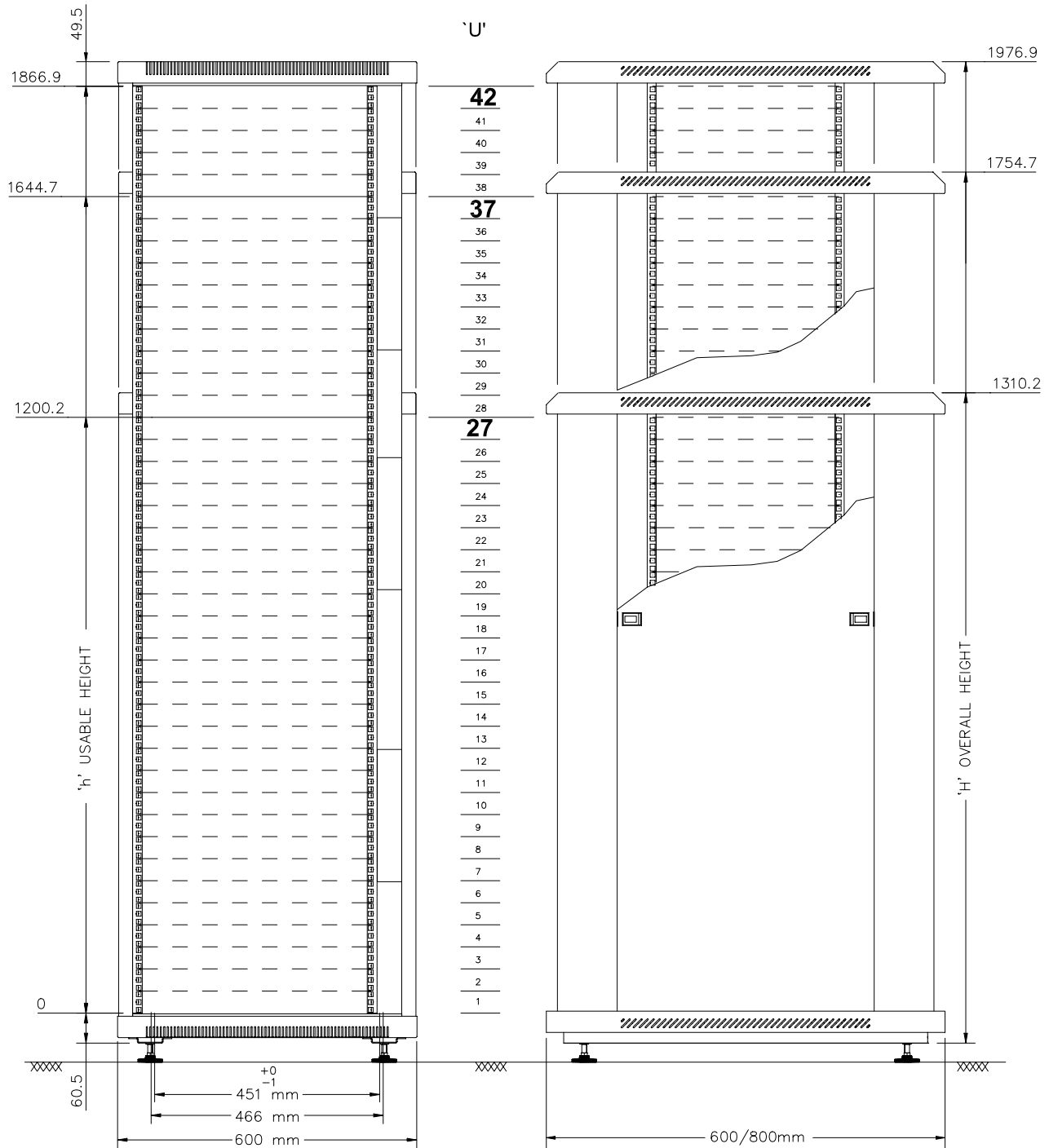
SIDE VIEW
